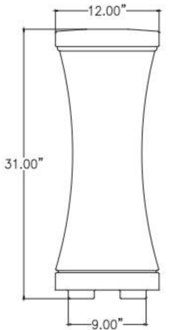
ELEVATION VIEW
