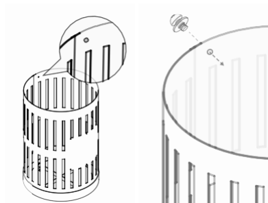
3. Identify mounting hole on base Remove and set aside liner. Identify predrilled hole in base. Insert supplied screw and washer with threads facing IN.
