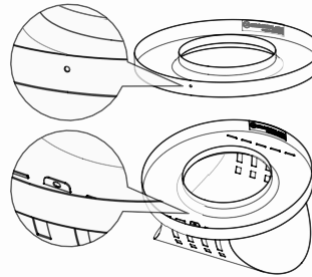
1. Identify predrilled hole in lid Open-Top lid: On underside of open-top lid, locate predrilled hole on outer ring. Canopy lid: On underside of canopy lid, locate tab with predrilled hole.
