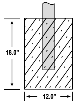
CONCRETE FOOTING
